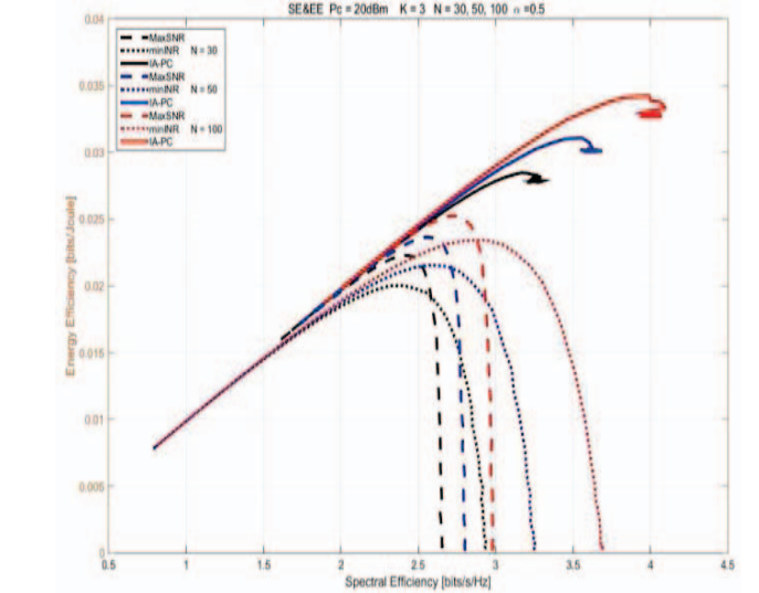
Fig. 2. Trade-off between SE and EE for varying the number of users in a cell when P_c=20 dBm, K=3 , and \alpha=0.5 .
